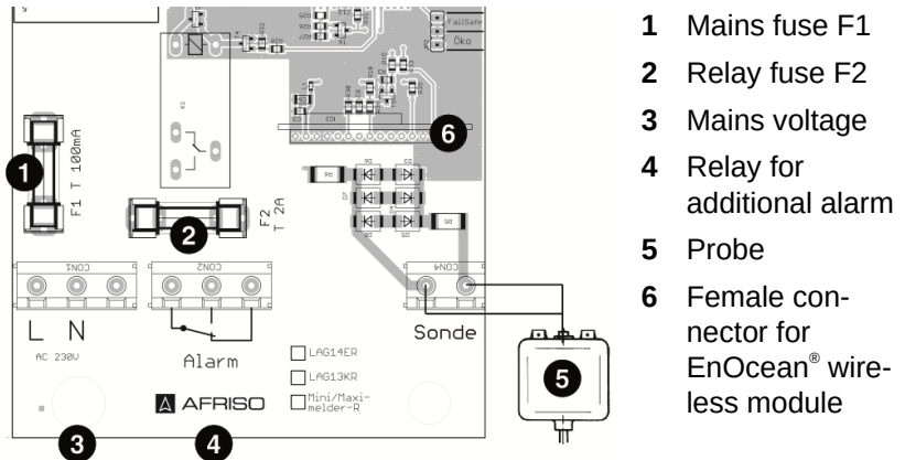
Fig. 6: Electrical connection
